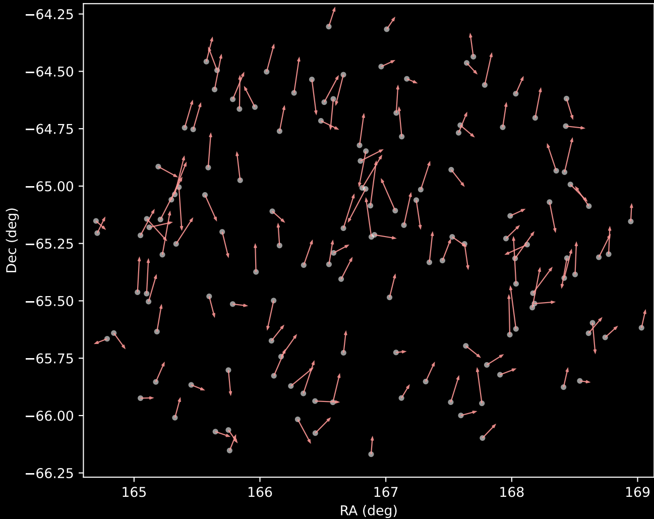
GALAH DR4 Cluster 7 Proper Motion Vectors (n=139)
