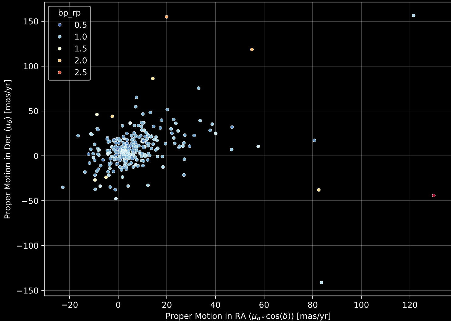
GALAH DR4 Field: [263] Proper Motion Diagram (n= 298)
