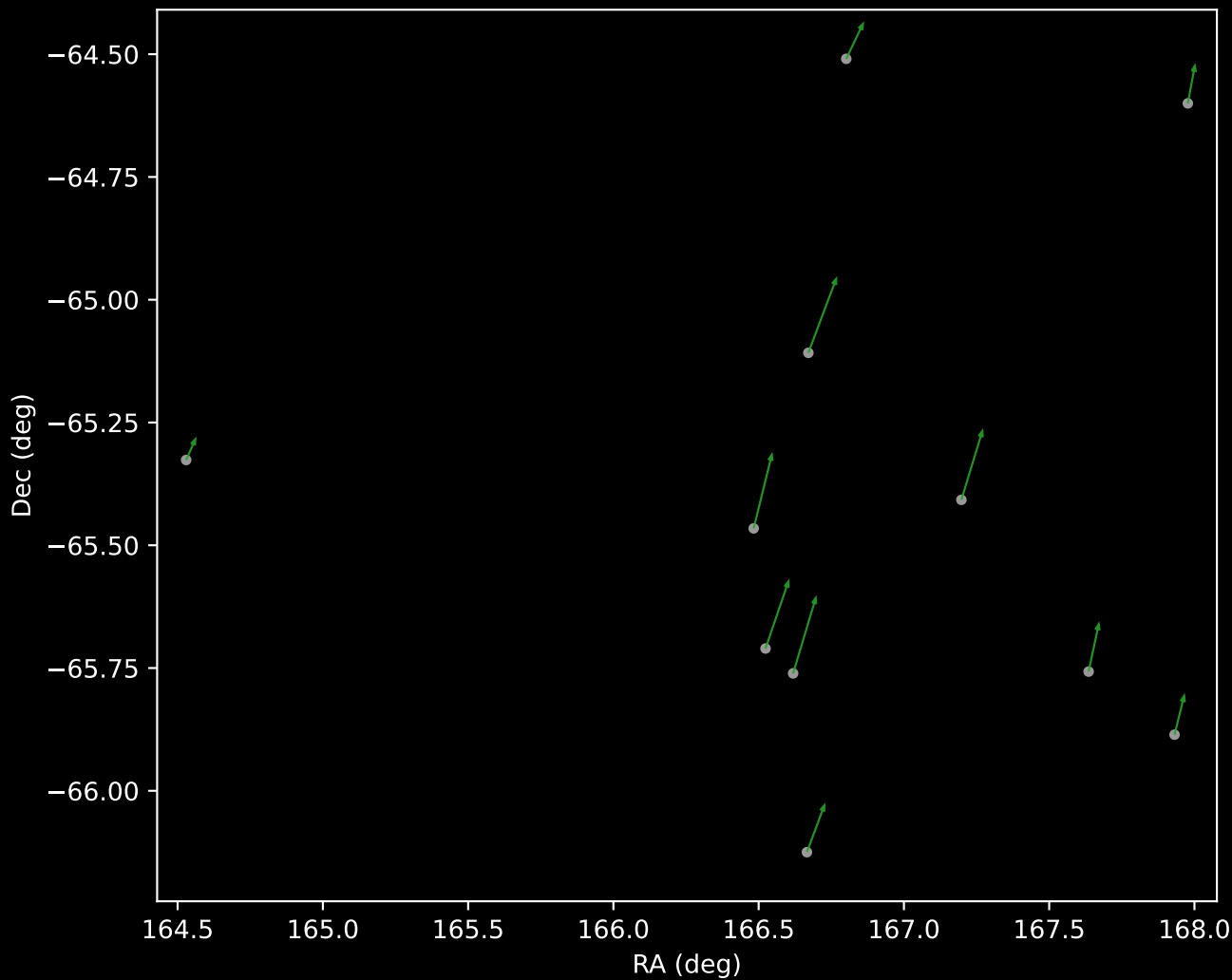
GALAH DR4 Cluster 4 Proper Motion Vectors (n=11)
