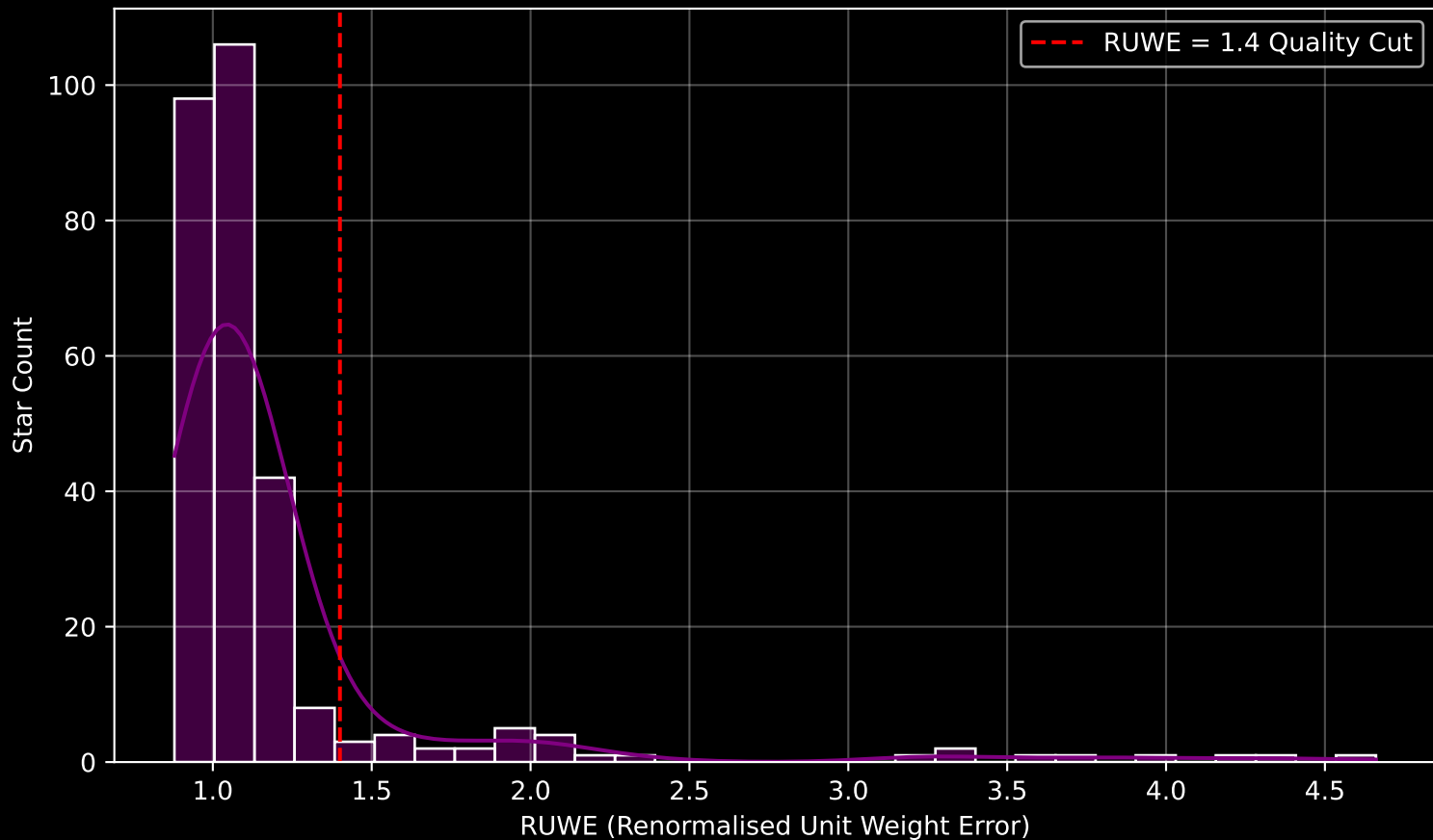
GALAH DR4 Field [263] RUWE Distribution (n= 285)
