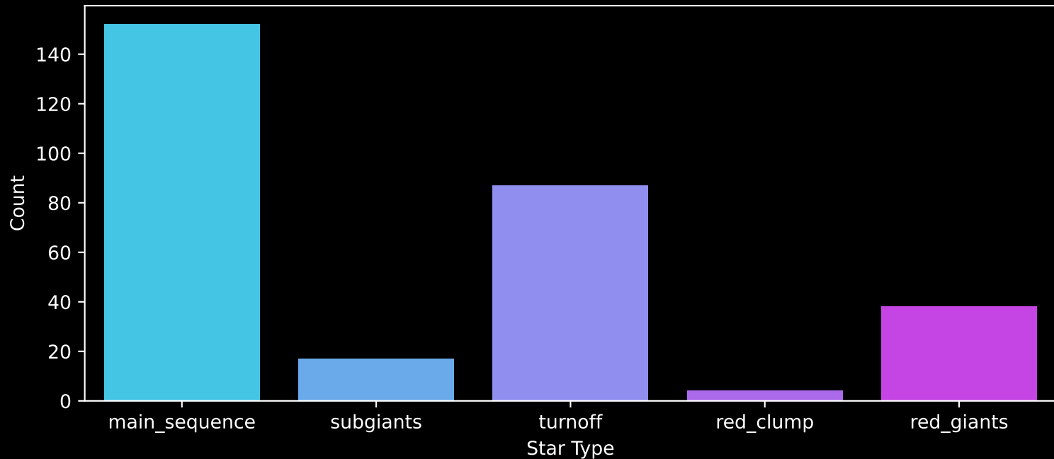
GALAH DR4 Field: [263] Count plot of Star Type
